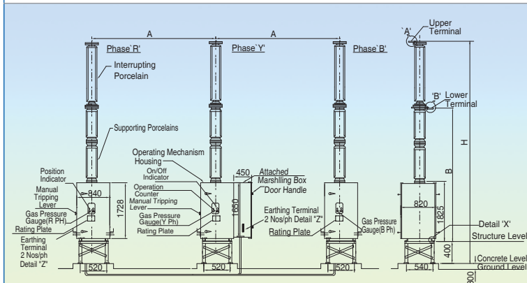
245kV Single Phase Auto Reclosing Breaker (40kA)
