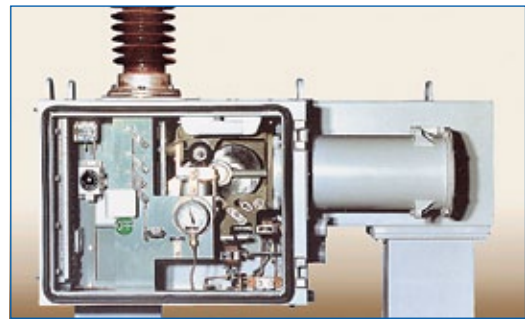
Spring Mechanism 145kV - Closing Spring
