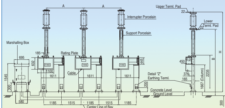
170kV Three Phase Auto Reclosing Breaker
