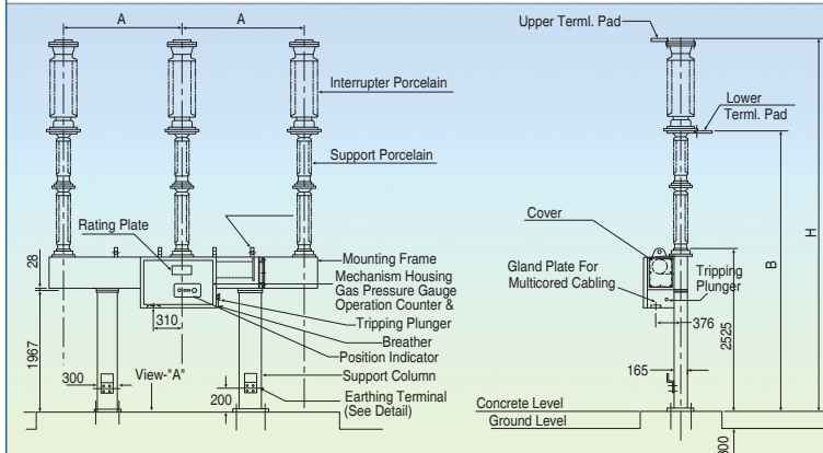
170kV Single Phase Auto Reclosing Breaker
