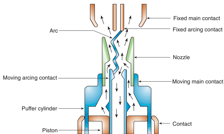
FIG. 3 : Interrupting principle
