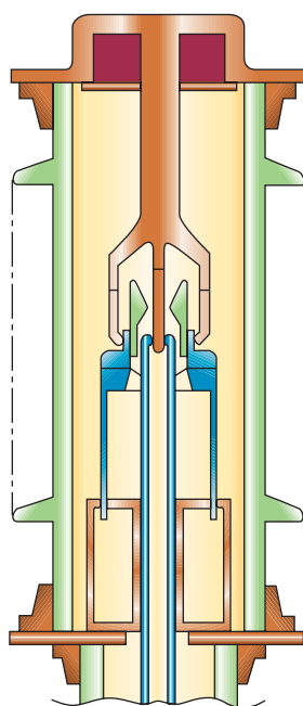
FIG. 1 : Closed position
