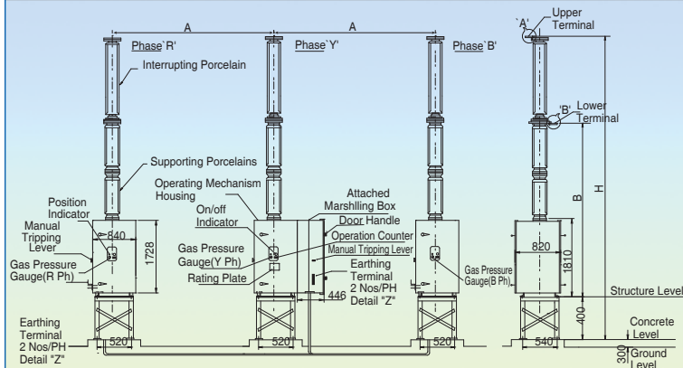
245kV Single Phase Auto Reclosing Breaker (40kA)
