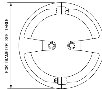
Corona Ring 230 kV to 400 kV
